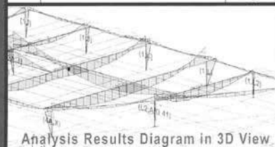
Curve Beam with Torsion Detailing
