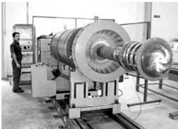
Dynamic Balancing Machine
