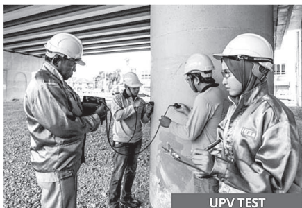
UPV TEST
